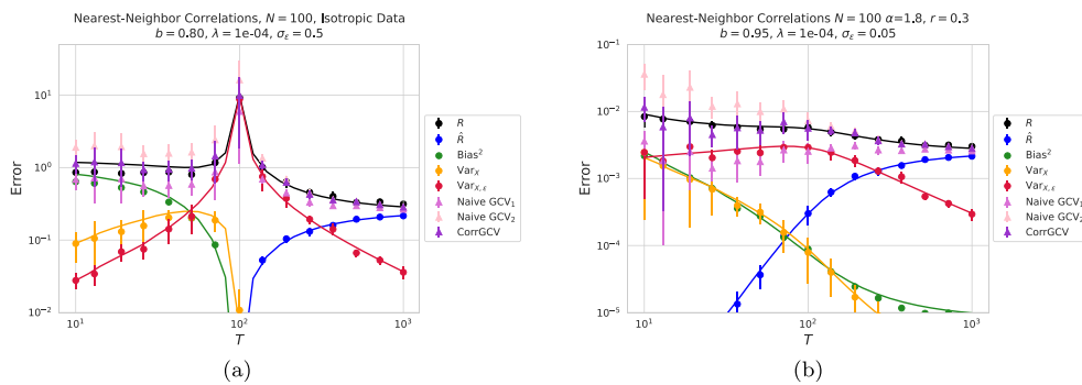
Figure 15. Risks, sources of variance, and risk estimators, similar to figure 1, but with nearest neighbor correlations. (a) Isotropic covariates. (b) Structured covariates under source and capacity conditions.
