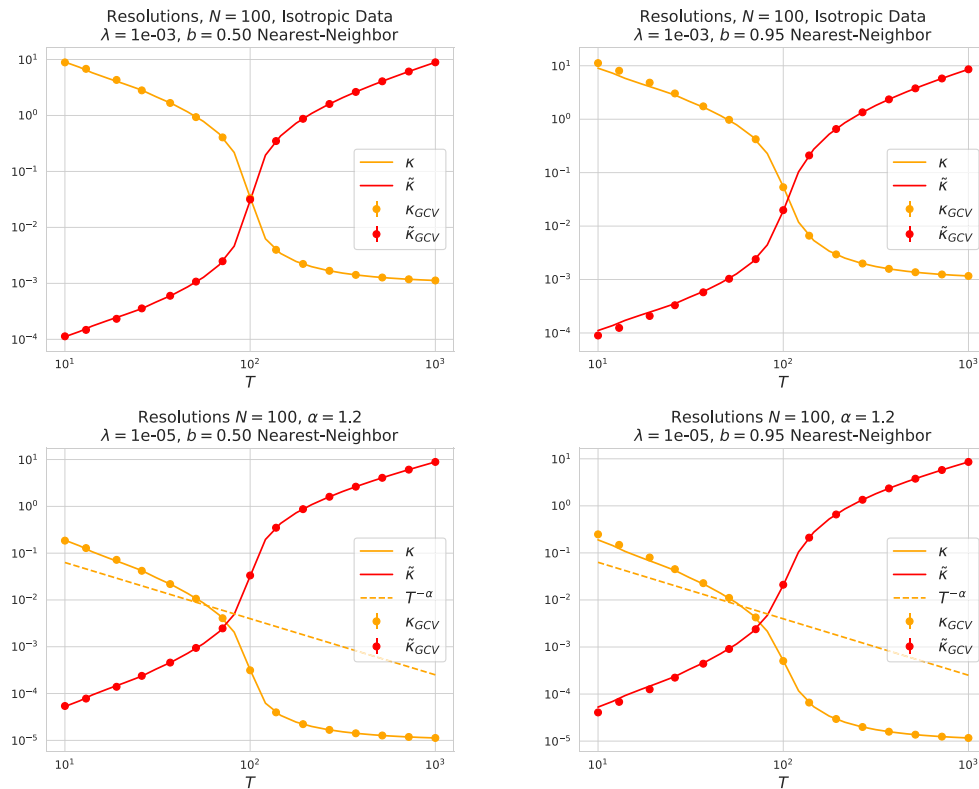
Figure 16. Plots of the resolution \kappa, \tilde{\kappa} under nearest neighbor correlations. Top: Isotropic data. Bottom: Anisotropic power law data with the eigenvalues of \Sigma having power law decay k^{-\alpha} , \alpha = 1.2 . Left: b = 0.5 , weakly correlated. Right: b = 0.95 , strongly correlated. We fix N = 100 and vary T . Solid lines are theory, dots with error bars are empirics. Overlaid in dashed is the expected scaling in the overparameterized regime when \alpha > 1 .
