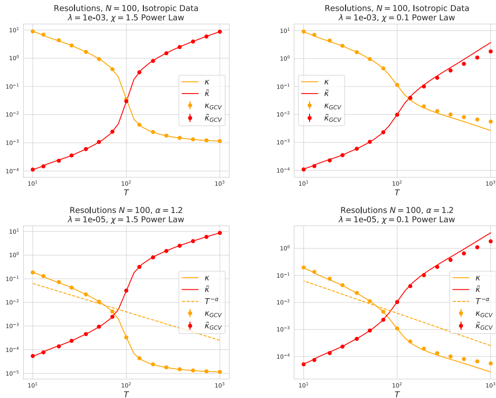
Figure 19. Plots of the resolution \kappa, \tilde{\kappa} under power law correlations. Top: Isotropic data. Bottom: Anisotropic power law data with the eigenvalues of \Sigma having power law decay k^{-\alpha} , \alpha = 1.2 . Overlaid in dashed is the expected scaling in the overparameterized regime. Left: \chi = 1.5 , weakly correlated. Right: \chi = 0.1 , strongly correlated. We fix N = 100 and vary T . For strongly correlated data, we see a slight deviation between \kappa in theory and empirics. This is due to the low-degree polynomial interpolation estimator of S_K(qdf_1) performing more poorly near qdf_1 = 1 . This can be resolved with a more flexible interpolant.
