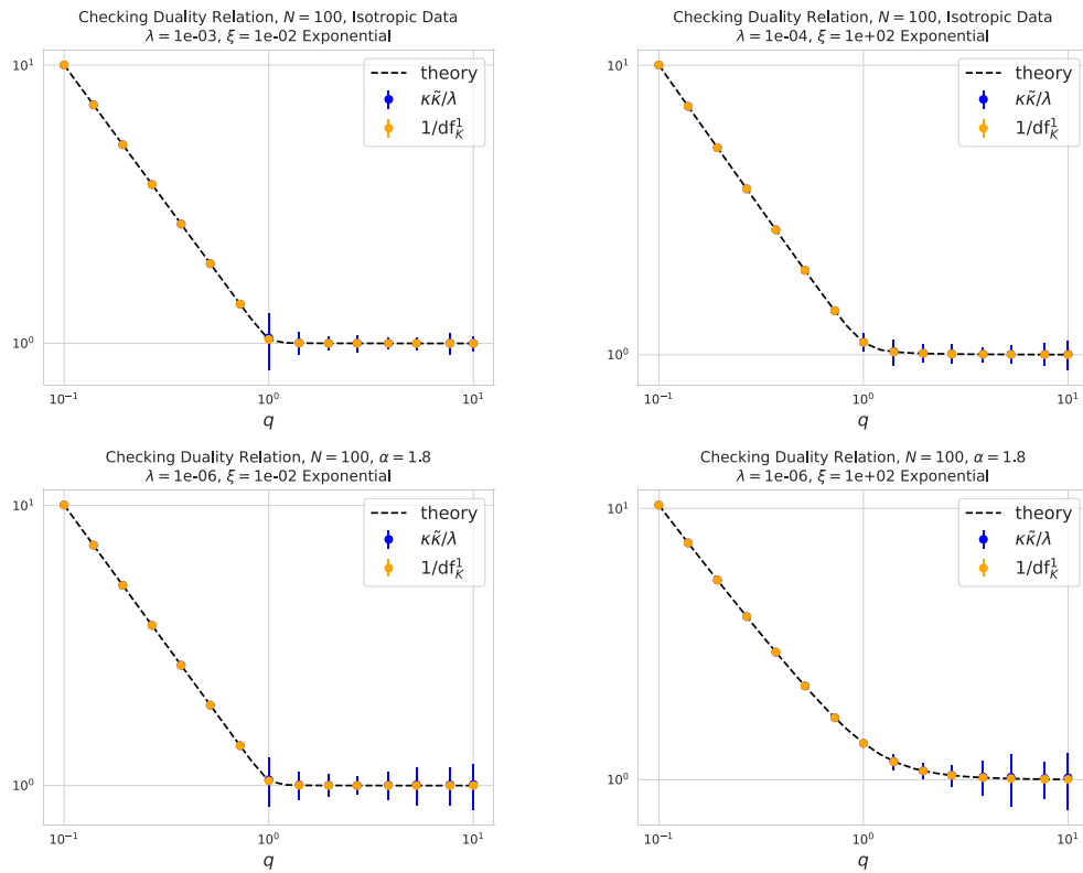
Figure 14. Plots verifying the duality relation \frac{\kappa\tilde{\kappa}}{\lambda} = \frac{1}{\text{df}_1} hold for the settings in figures 12 and 13 under exponential correlations. Dashed black lines are theory, dots with error bars are empirics. The lack of substantial error bars stems from the fact that all quantities concentrate.
