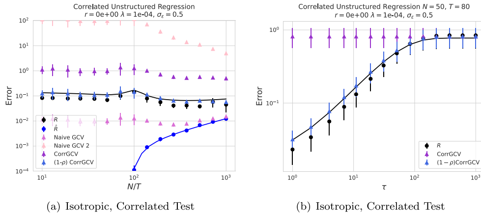
Figure 6. Strongly exponentially correlated data as in figure 1(b), with \mathbb{E}\mathbf{x}_t\mathbf{x}_{t+\tau} \sim e^{-\tau/\xi} , \xi = 10^2 . (a) Comparison of the out-of-sample risk for testing on a correlated point that is \tau = 5 time points in the future from the training data. We emphasize that the CorrGCV here is the CorrGCV for testing on an uncorrelated test point, which is pessimistic relative to the risk for the correlated point at \tau = 5 . (b) Plot of the out-of-sample risk as a function of the horizon time that we test out. We see that testing on closer times is predictably more optimistic. We see that (1 - \rho) times the CorrGCV provides a good approximation of the optimism of testing on a correlated point. Given a knowledge of the correlation structure of \mathbf{K} , this can be efficiently computed for stationary time series data.
