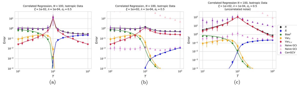
Figure 4. Precise asymptotics for double descent in linear regression with unstructured data across various correlations. We choose an exponential correlation with correlation length \xi and vary \xi . (a) Weakly correlated data and noise, giving rise to the traditional double descent curve as analyzed in [11, 45]. All GCV-related estimators agree and correctly estimate the out-of-sample risk. (b) Strongly correlated data with matched noise correlations. The double descent peak is mollified . (c) Strongly correlated data but uncorrelated noise. The double descent peak is exacerbated . This mismatch in correlations violates the assumptions of the CorrGCV, and thus no GCV can asymptotically match it without knowledge of the noise level \sigma_\epsilon . Across all settings the theory curves (solid lines) find excellent agreement with the experiments (solid markers with error bars over 10 different datasets).
