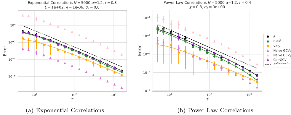
Figure 3. Power law scalings for data with (a) exponential correlations with \xi = 10^2 and (b) power law correlations \mathbb{E}\mathbf{x}_t^\top \mathbf{x}_{t+\tau} \propto \tau^{-\chi} with \chi = 0.3 . In both cases, the correlations of the data do not affect the scaling of the generalization error as a function of T , which generally goes as T^{-2\alpha\min(r,1)} , as derived in prior works. Although other estimators correctly predict the rate of decay, only the CorrGCV correctly recovers the exact risk.
