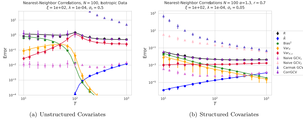
Figure 11. Plot of the Carmack et al [28] estimator relative to other GCV estimators defined earlier. We note that similar to the naive GCVs 1 and 2, the Carmack estimator fails to correctly predict R . (a) Unstructured covariates. (b) Structured covariates with source and capacity exponents as labeled.
