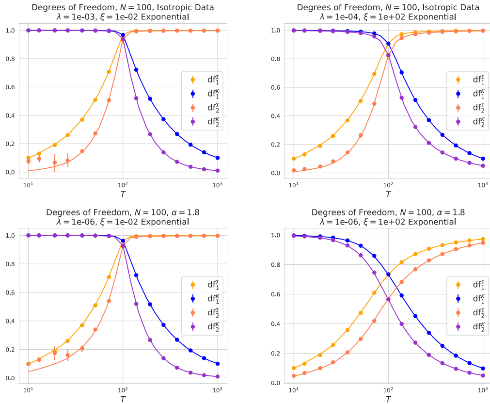
Figure 13. Plots of the degrees of freedom df_1, \tilde{df}_1, df_2, \tilde{df}_2 under exponential correlations as in figure 12. Solid lines are theory, dots with error bars are empirics. The lack of substantial error bars stems from the fact that all quantities concentrate. We find that although df_2 can be numerically sensitive, \tilde{df}_2 remains numerically precise even in the presence of strong correlations.
