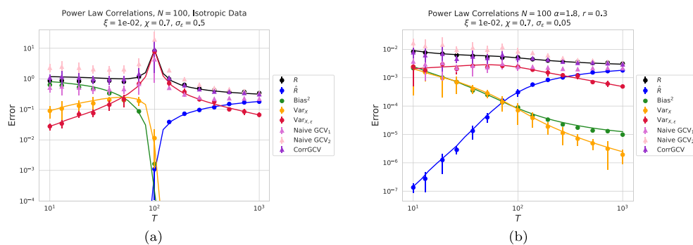
Figure 18. Risks, sources of variance, and risk estimators, similar to figure 1, but with power law correlations \mathbb{E}[\mathbf{x}_t \cdot \mathbf{x}_s] \propto (1 + |t - s|)^{-\chi} with exponent \chi = 0.7 . (a) Isotropic covariates. (b) Structured covariates under source and capacity conditions.
