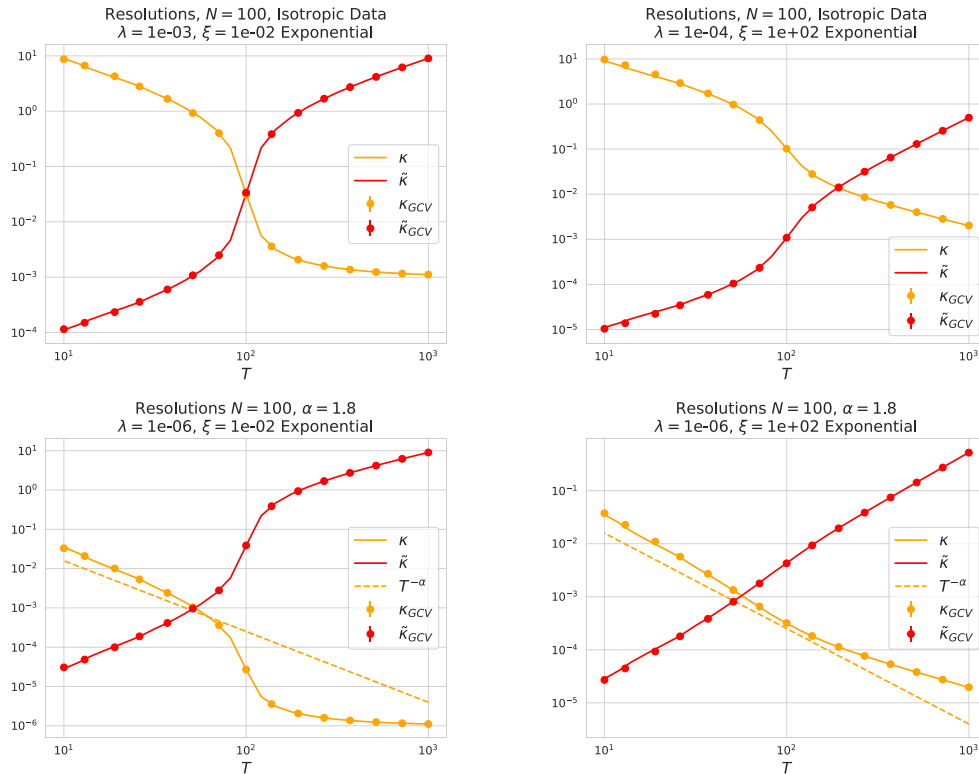
Figure 12. Plots of the resolutions \kappa, \tilde{\kappa} under exponential correlations. Top: Isotropic data. Bottom: Anisotropic power law data with the eigenvalues of \Sigma having power law decay k^{-\alpha} , \alpha = 1.8 . Overlaid in dashed is the expected scaling in the overparameterized regime. Left: \xi = 10^{-2} , essentially uncorrelated. Right: \xi = 10^2 , strongly correlated. We fix N = 100 and vary T . Overlaid in dashed is the scaling expected in the overparameterized regime when \alpha > 1 .
