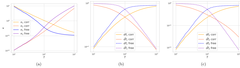
Figure 10. Theory curves comparing \kappa, \tilde{\kappa}, df_1, \tilde{df}_1, df_2, \tilde{df}_2 for correlated data \mathbf{K} \neq \mathbf{I} vs uncorrelated data \mathbf{K} = \mathbf{I} at \lambda = 10^{-1} for N = 100 on isotropic data. For the correlations, we choose exponential correlations with length \xi = 10^2 . (a) We see across the board that in the presence of explicit ridge, \kappa grows while \tilde{\kappa} shrinks under correlations. (b) We see that the df_1, \tilde{df}_1 are always decreased by the presence of correlations when the ridge is present. (c) We see a similar behavior for df_2 . For \tilde{df}_2 , we also see a decrease in the neighborhood of the double descent peak T = N . Still, at first order near T = N , we see agreement of \tilde{df}_2 between the correlated and uncorrelated settings, as predicted by our theory.
