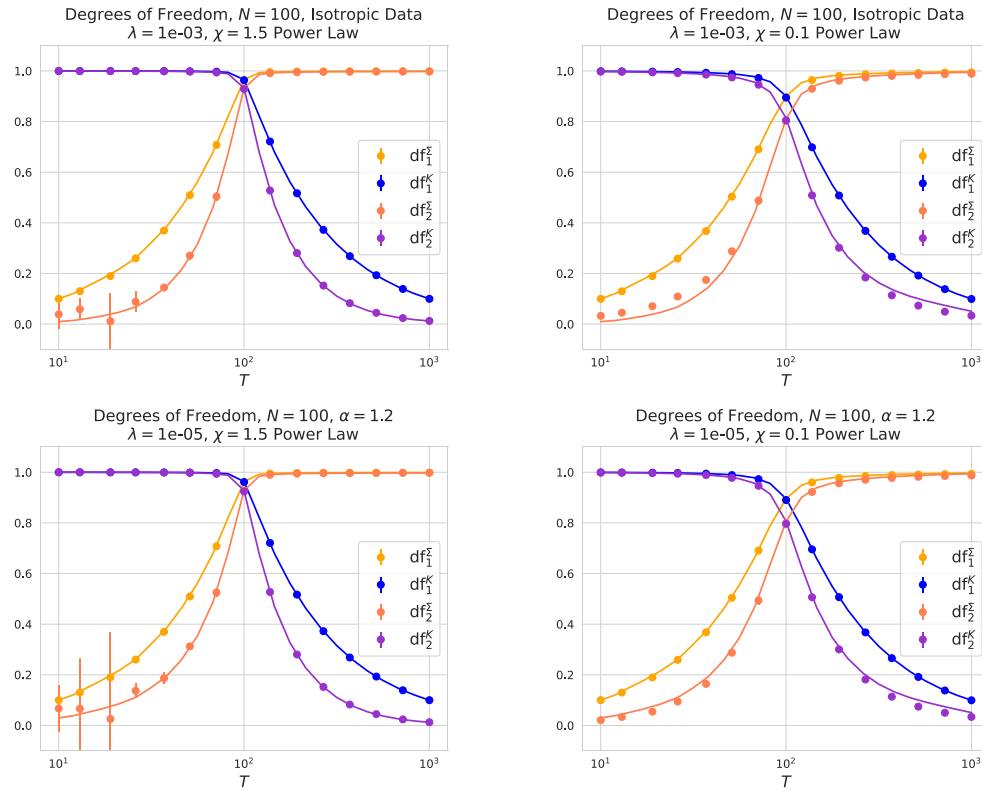
Figure 20. Plots of the the degrees of freedom df_1, \tilde{df}_1, df_2, \tilde{df}_2 under power law correlations as in figure 19. Solid lines are theory, dots with error bars are empirics. The lack of substantial error bars stems from the fact that all quantities concentrate. We find that although df_2 can be numerically sensitive, \tilde{df}_2 remains numerically precise even in the presence of strong correlations.
