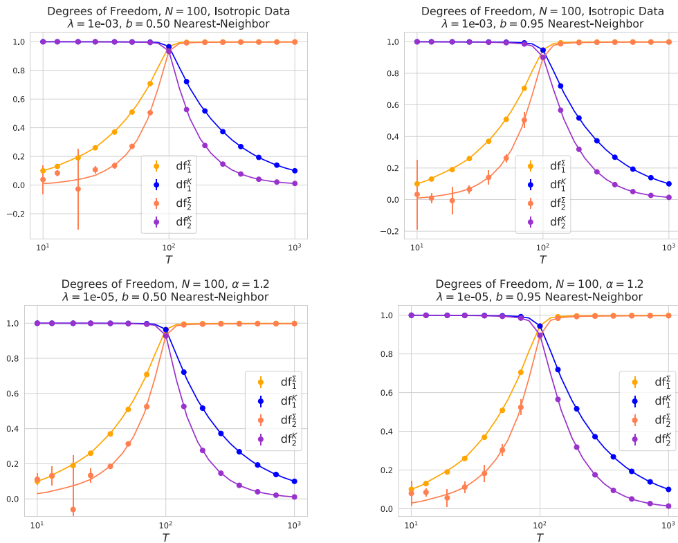
Figure 17. Plots of the the degrees of freedom df_1, \tilde{df}_1, df_2, \tilde{df}_2 under nearest-neighbor correlations as in figure 16. Solid lines are theory, dots with error bars are empirics. The lack of substantial error bars stems from the fact that all quantities concentrate. We find that although df_2 can be numerically sensitive, \tilde{df}_2 remains numerically precise even in the presence of strong correlations.
